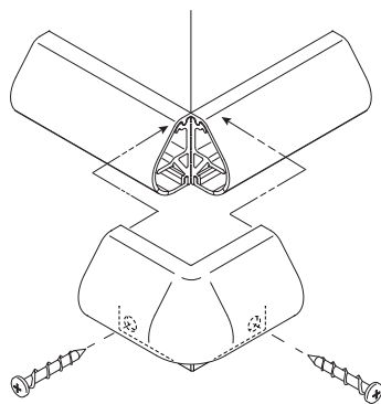
Outside Corner Cover
