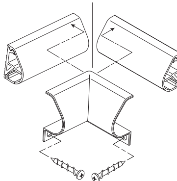
Inside Corner Cover
